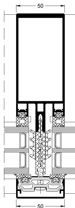
Facciata Schüco FWS 50 Green, Scala 1:2 Schüco façade FWS 50 Green, Scale 1:2
