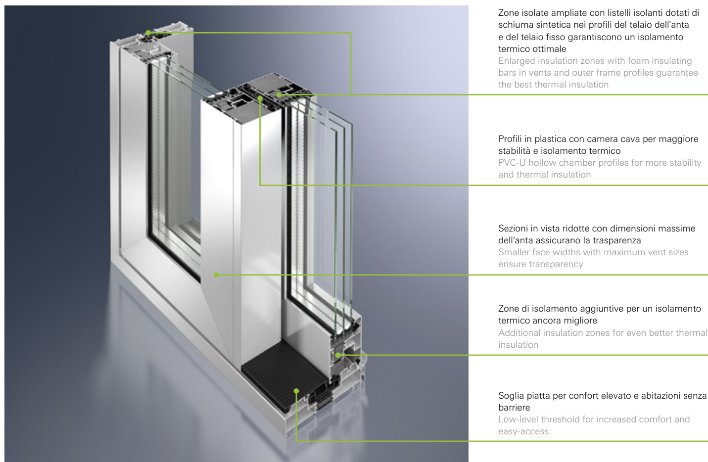
Sistema scorrevole a sollevamento e scorrevole a elevato isolamento termico ASS 70.HI Schüco ASS 70.HI highly thermally insulated sliding and lift-and-slide system
