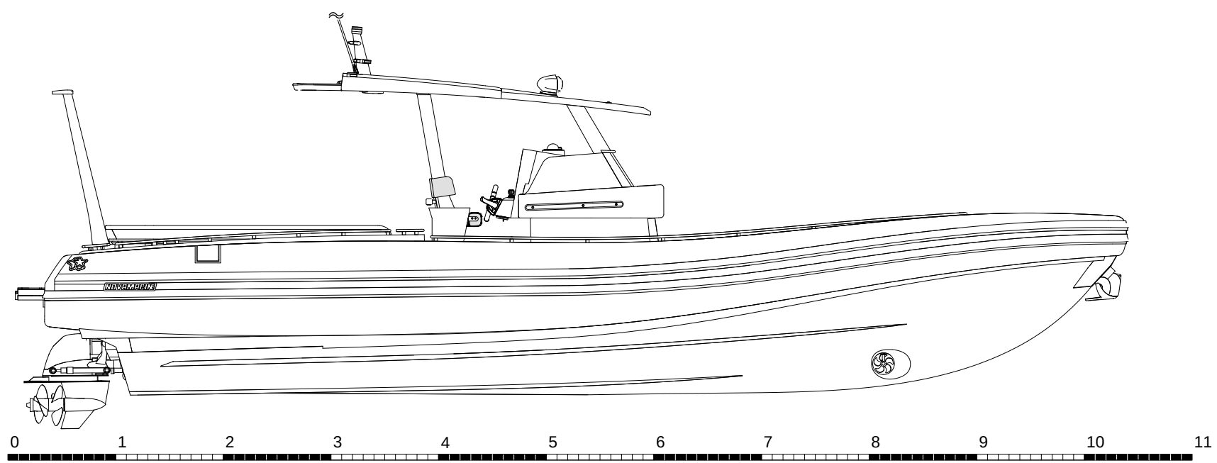
SIDE VIEW
