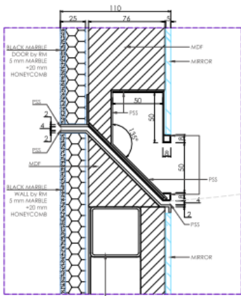
(18) Detail Scale 1:5
