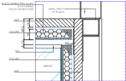
(19) Detail Scale 1:2
