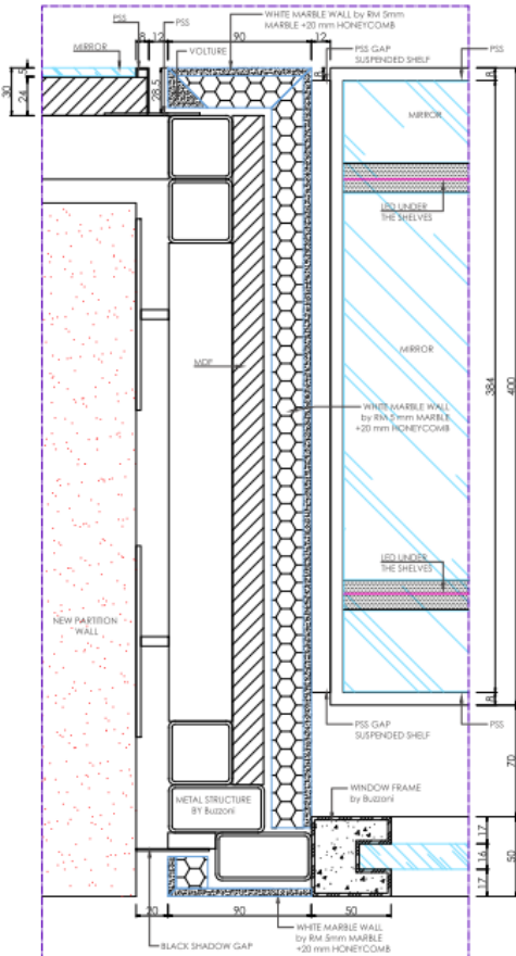
(2) Detail Scale 1:2
